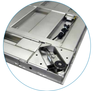
Detail of load cell mounting
